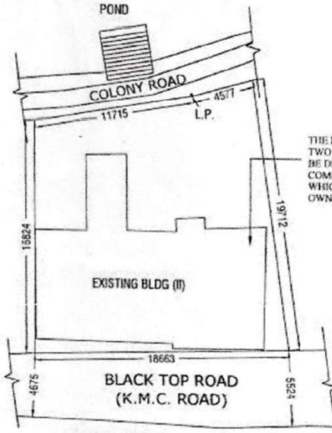
EXISTING BUILDING PLAN SCALE:- 1:200
